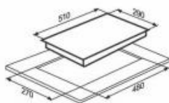
30cm Built-in Induction Cooker Hob
