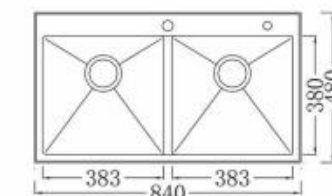
Topmount Handcrafted Kitchen Sink
