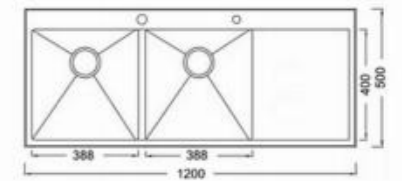
Topmount Handcrafted Kitchen Sink
