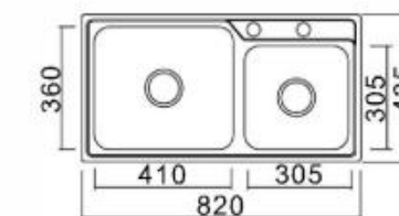
Topmount Kitchen Sink
