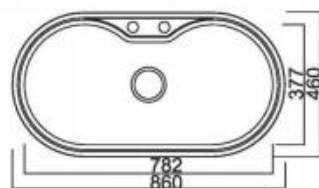
Topmount Kitchen Sink
